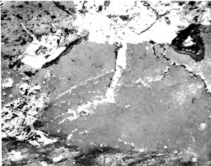
Fig. 23—Polished surface of ore, showing veinlets of sulphides (white) replacing or impregnating rock; magnified 88 diameters; Creighton mine, Sudbury area, Ontario. The sulphides replace or impregnate all the rocks at Creighton mine, whether they consist of norite, granite or greenstone. Photomicrograph by Wm. Campbell.
